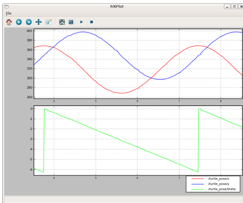
Figure 21: rxplot of /Example node with its topics
