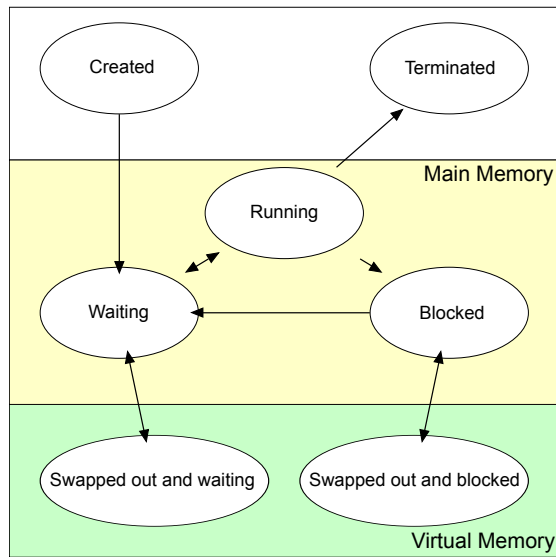
Figure 23: Processus Transitions
