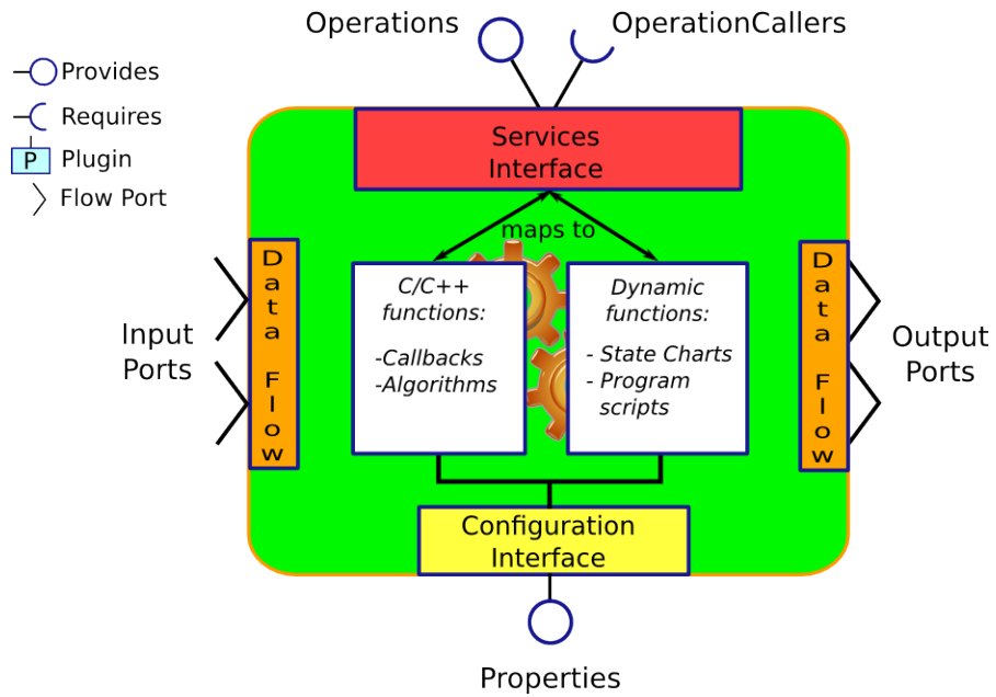
Figure 13: Component Description
