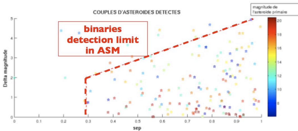
Fig. 2 – Binaries detection limit in ASM. Simulation form a synthetic population as a function of separation and magnitude difference (credit J. Blanchot).
