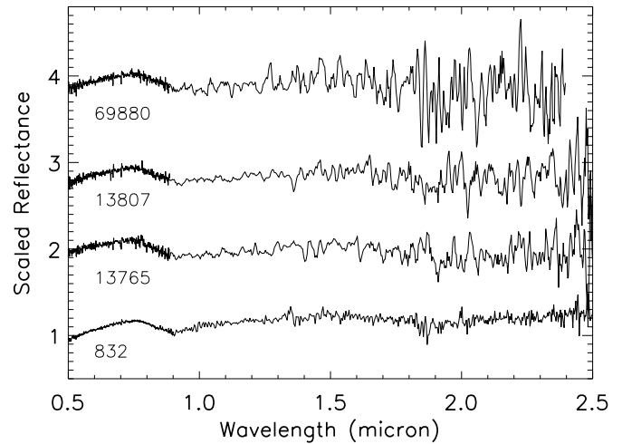
Fig. 4. Spectra of 832, 13765, 13807, and 69880 in the 0.5\text{--}2.5 \mu\text{m} range. The spectra were vertically displaced for clarity. The NIR spectra have been brought to lower resolution by Gaussian smoothing. The Gaussian width used was 4 points.
