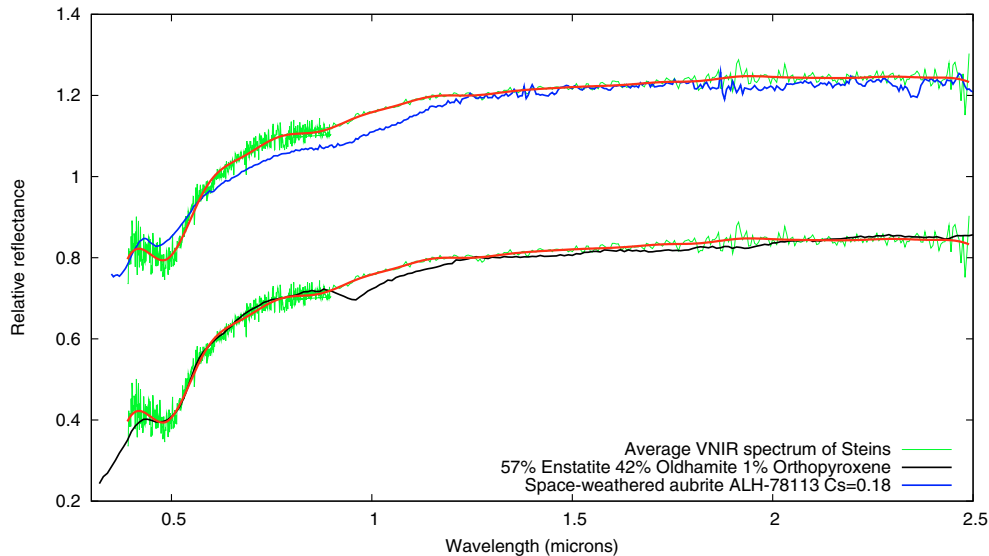
Fig. 2. The visible, plus averaged NIR, spectrum of (2867) Steins (green line) smoothed with a bicubic spline function (red line). The spectrum was fitted with a linear (areal) mix of three components taken from the RELAB database as presented in the text (black). The second fit represents a modeled space-weathered spectrum of the aubrite ALH-78113 (blue).
