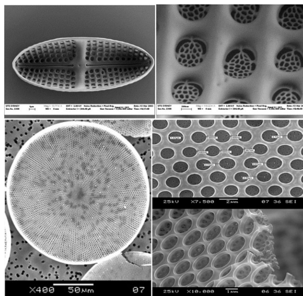
Fig. 4 Hierarchical distribution of pores in diatom frustules; Top: Achmanthes subsessilis (reprinted from Materials Science and Engineering C, 25, K.S.A. Butcher et al. , A luminescence study of porous diatoms, 659, Copyright (2010), with permission from Elsevier); Bottom: Coscinodiscus walesii (reprinted from ref. 77, Copyright (2010), with permission from Elsevier).
