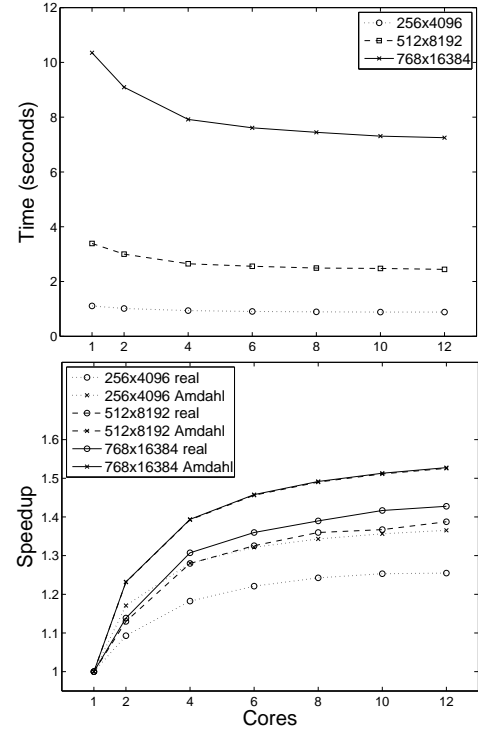
Fig. 15. Marine acoustics performance measurements for three 2D computational space sizes over one time step (time averaged over 30 time steps). The time encompasses both the forward and the backward procedures.
