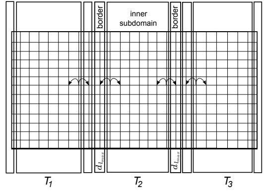
Fig. 7. Subdomain decomposition with d_{lmax} = 1 for threads T_1 , T_2 and T_3 . Each thread domain is decomposed into two border subdomains with d_{lmax} grid points in the parallel dimension, and one inner subdomain.
