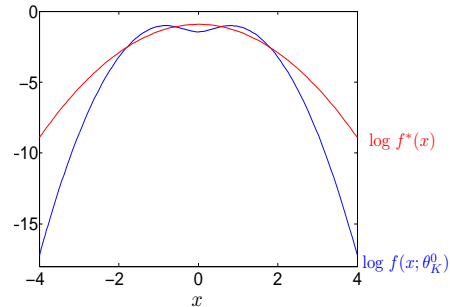
Figure 5: \log f^\varphi (red, which is also \log f(\cdot; \theta_2^{KL}) ) and \log f(\cdot; \theta_2^0) (blue) for Example 2.1
