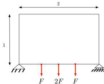
FIGURE 15. Boundary conditions for the 3-force bridge.
