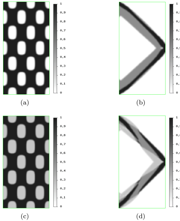
FIGURE 14. Short cantilever using two or three phases and void; (a) initialization for two phases and void, (b) optimal shape for two phases and void, (c) initialization for three phases and void, (d) optimal shape for three phases and void.
