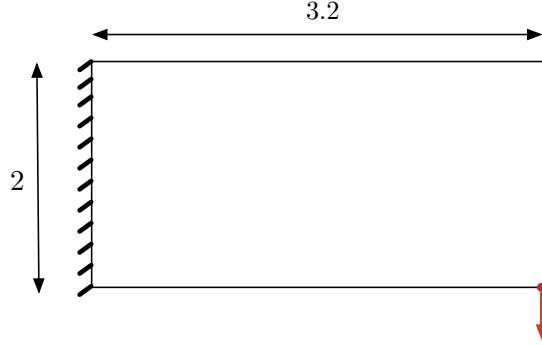
FIGURE 17. Boundary conditions and initialization for the medium cantilever.
