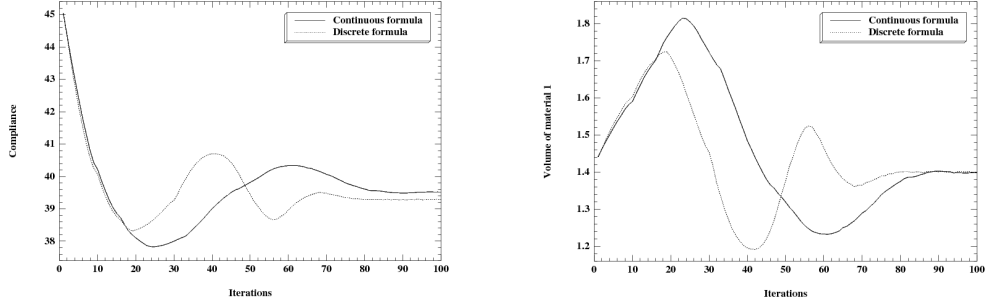
FIGURE 10. Convergence history of the compliance (left) and the volume (right) for the sharp interface results displayed on Figure 9.
