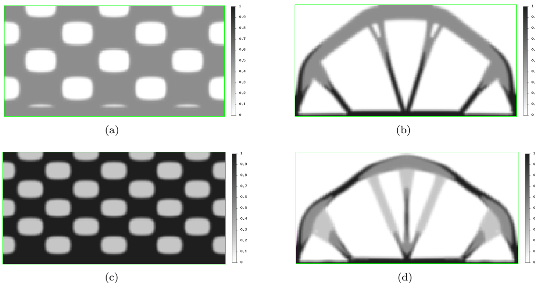
FIGURE 16. 3-force bridge using two or three phases and void; (a) initialization for two phases and void, (b) optimal shape for two phases and void, (c) initialization for three phases and void, (d) optimal shape for three phases and void.
