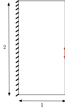
FIGURE 13. Boundary conditions and initialization for the short cantilever.
