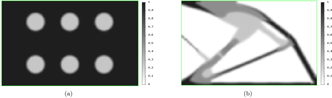
FIGURE 18. Medium cantilever using three materials and void; (a) initialization, (b) optimal shape.
