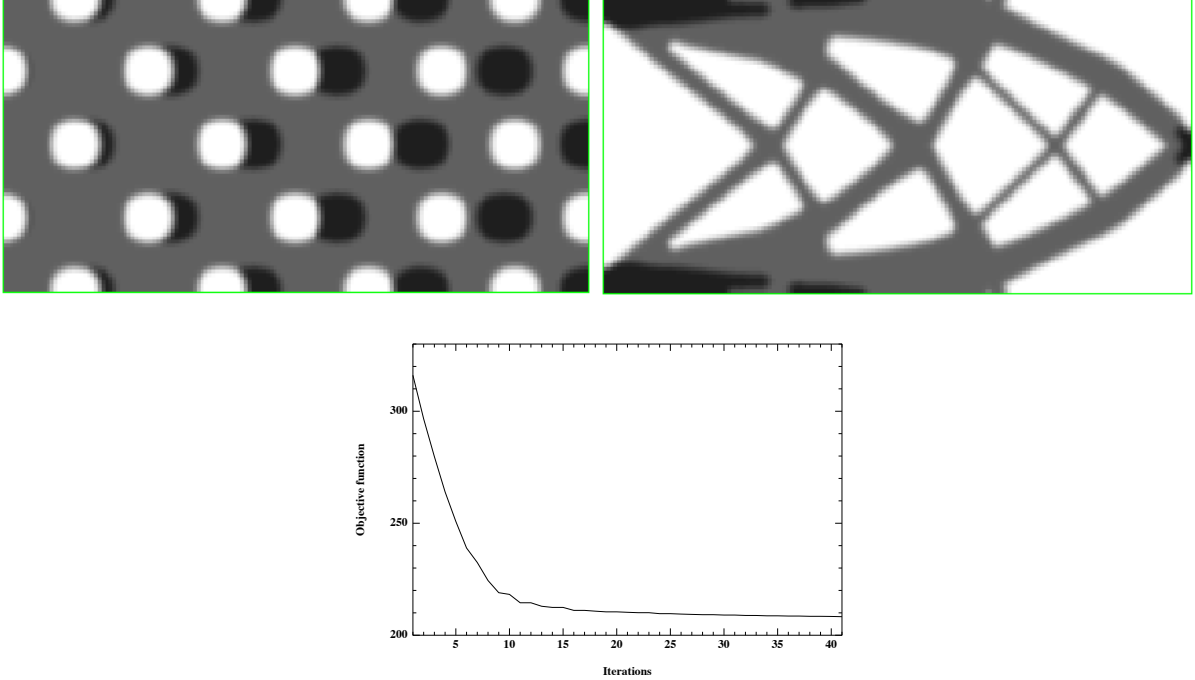
FIGURE 19. Initialization with two materials (top left), optimal shape (top right) and convergence history of the objective function (bottom).
