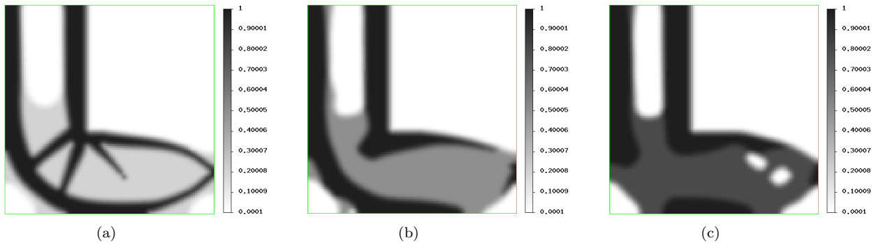
FIGURE 22. Results for the L-beam with varying second phase.
