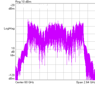
Fig. 7. Spectrum of received signal in NLOS scenario.
