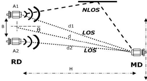
Fig. 5. RD and MD configuration in NLOS Scenario.
