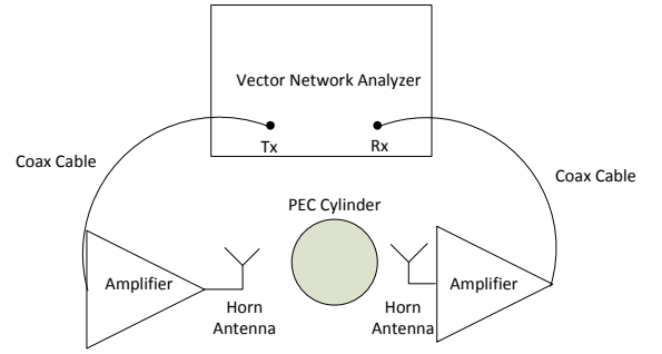
Fig. 6. TM mode Experimental set-up
