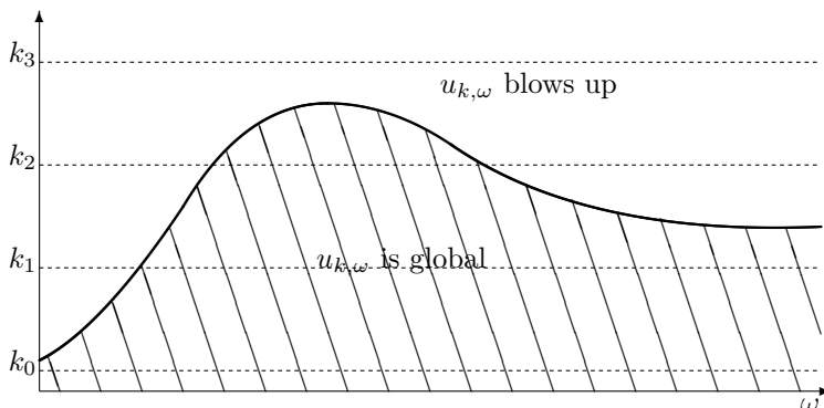
FIGURE 1. The \omega, k picture of Theorem 1.6
