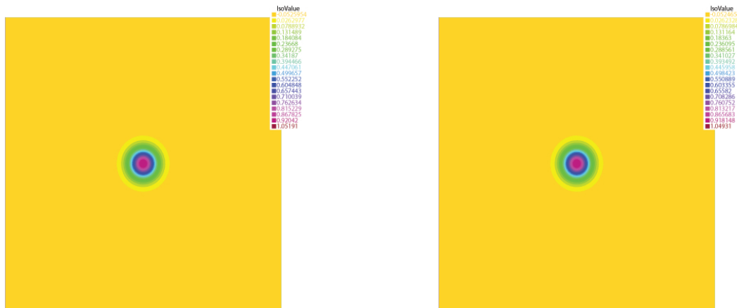
FIGURE 11. Exact solution (left) and numerical solution (right) after the mesh refinement for \lambda = 10 and p = 1 .
