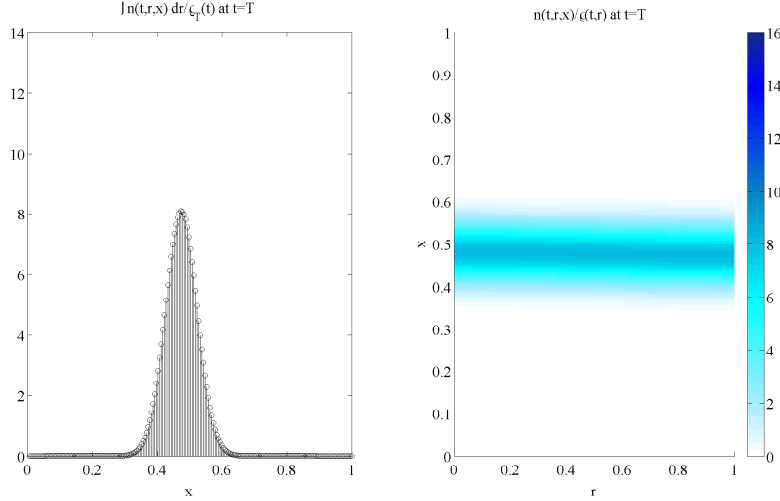
Figure 5: (Cell dynamics under constant infusion of cytostatic drugs) Plots of the average resistance trait distribution \int_0^1 n(T, r, x)dr/\varrho_T(T) (left panel) and the phenotype distribution along the tumor radius n(T, r, x)/\varrho(T, r) (right panel) for C_1(t) := 0 and C_2(t) := 1 . Cytostatic drugs slow down the evolution of cancer cells and do not favor the emergence of resistance
