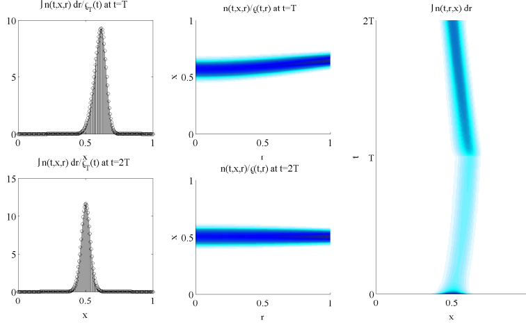
Figure 4: (On-off switch of cytotoxic drug infusion) Plots of \int_0^1 n(T, r, x)dr/\varrho_T(T) (left-top panel), \int_0^1 n(2T, r, x)dr/\varrho_T(2T) (left-bottom panel), n(T, r, x)/\varrho(T, r) (center-top panel), n(2T, r, x)/\varrho(2T, r) (center-bottom panel) and \int_0^1 n(t, r, x)dr for t \in [0, 2T] (right panel), for C_1(t) defined by (3.1) and C_2(t) := 0 . The selection of higher levels of resistance occurs during the infusion of cytotoxic drugs, i.e., in time interval [0, T] , while higher levels of proliferative potential are selected in the absence of cytotoxic drugs, i.e., in time interval (T, 2T] .
