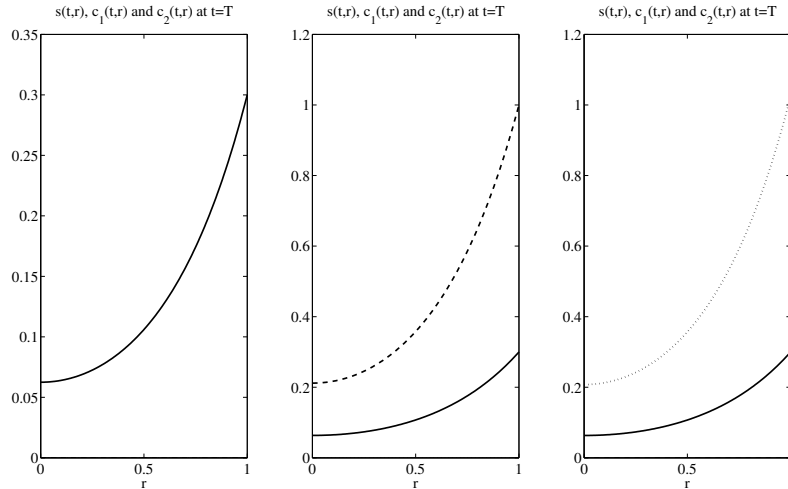
Figure 2: (Distributions of resources and drugs) Plot of s(T, r) (solid lines), c_1(T, r) (dashed lines) and c_2(T, r) (dotted lines) for C_{1,2}(t) := 0 (left panel), C_1(t) := 1, C_2(t) := 0 (center panel) and C_1(t) := 0, C_2(t) := 1 (right panel).
