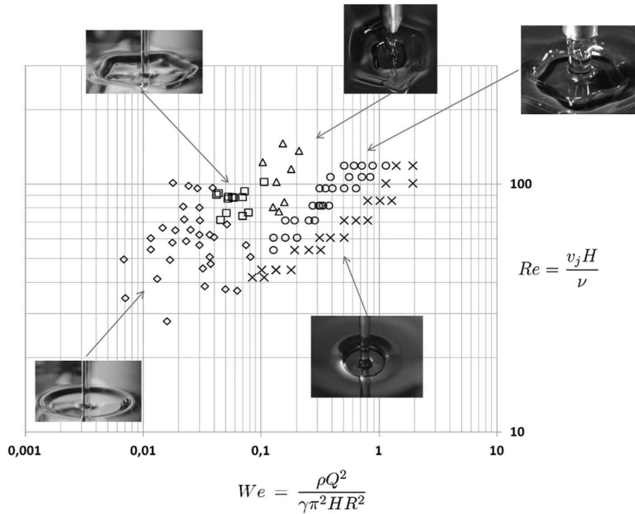
FIG. 5. The dependence of the flow structure on Reynolds number Re = (v_j H)/\nu and Weber number We = \rho Q^2 / (\gamma \pi^2 H R^2) , where v_j = Q/(2\pi R_n) is the jet speed, and R the radius of the bump or jump. ( \diamond ): Circular bumps observed for viscosities in the range of \nu = 58 – 96 cS. ( \square ): Polygonal bumps ( \nu = 58 – 96 cS) with number of sides ranging from 5 to 10. ( \triangle ): The double jump structure for which a polygonal jump is enclosed by a polygonal bump. ( \times ): Circular type I jumps ( \nu = 10 cS from Bush et al. 14 ). ( \circ ): Polygonal jumps with 3 to 10 sides ( \nu = 10 cS, data from Bush et al. 14 ). Reprinted with permission from J. W. M. Bush, J. M. Aristoff, and A. E. Hosoi, J. Fluid Mech. 558 , 33–52 (2006). Copyright 2006, Cambridge University Press.
