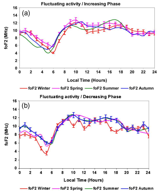
Fig. 5. foF2 variability under shock fluctuating geomagnetic activity during the sunspot increasing phase (a) and the sunspot decreasing phase (b). The blue curve corresponds to autumn, the red one to winter and the pink and green ones respectively to spring and summer.
