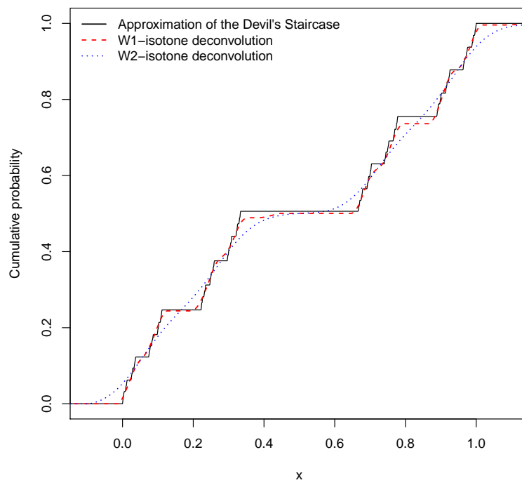
Figure 5: Approximation of the Devil's staircase and distributions functions of the W_1 and W_2 isotone deconvolution estimators.
