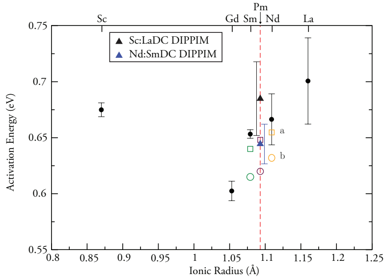
FIG. 7. DIPPIIM activation energies (eV) for \text{Ce}_{0.90}\text{RE}_{0.10}\text{O}_{1.95} from Figure 4 along with those for the co-doped systems, Nd:SmDC (filled blue triangle) and Sc:LaDC (filled black triangle). Experimental values from a) Omar et al. [37] (open squares) and b) Kasse and Nino [46] (open circles) with green for SmDC, maroon for Nd:SmDC and orange for NdDC.
