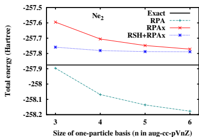
FIG. 1: (Color online) RPA, RPax and RSH+RPax total energies of Ne 2 at equilibrium distance (5.84 Bohr) with respect to the basis size.
