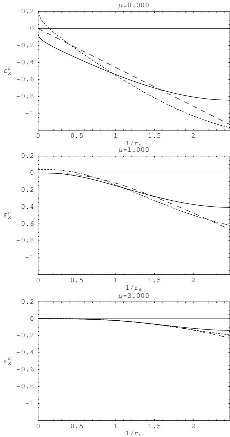
FIG. 4: Short-range local exchange energies per particle with respect to 1/r_s for He with the erf interaction for \mu = 0, 1, 3 : \bar{\epsilon}_x^{\mu,\text{LDA}} (long-dashed curve) is compared to the accurate \bar{\epsilon}_x^{\mu,\text{pd}} [Eq. (14), solid curve] and \bar{\epsilon}_x^{\mu,\text{local}} [Sec. (III B), short-dashed curve].
