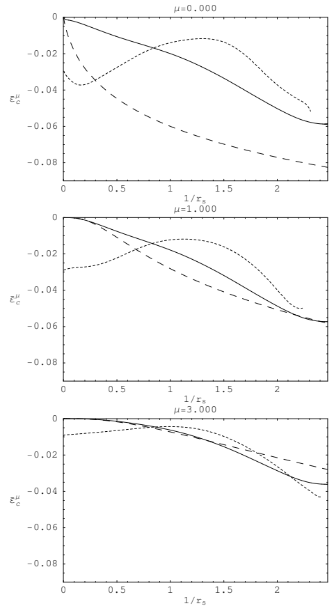
FIG. 5: Short-range local correlation energies per particle with respect to 1/r_s for He with the erf interaction for \mu = 0, 1, 3 . \bar{\epsilon}_c^{\mu,\text{LDA}} (long-dashed curve) is compared to the accurate \bar{\epsilon}_c^{\mu,\text{pd}} [Eq. (16), solid curve] and \bar{\epsilon}_c^{\mu,\text{local}} [Sec. (III B), short-dashed curve].
