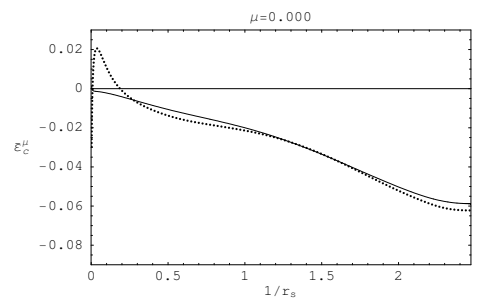
FIG. 6: Accurate local short-range correlation energies per particle \bar{\epsilon}_c^{\mu,\text{pd}} [Eq. (16)] with respect to 1/r_s for He with the erf (solid curve) and erfgau (dotted curve) interactions for \mu = 0 .
