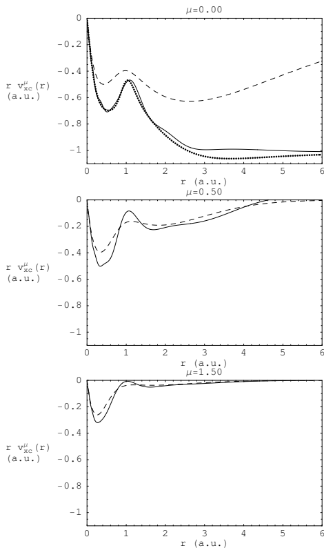
FIG. 3: Exchange-correlation potentials r v_{xc}^{\mu}(r) for Be with the erf interaction with \mu = 0, 0.5 and 1.5 : the potentials obtained in the present work (full curves) are compared to the LDA potentials [Eq. (10), dashed curves]. For \mu = 0 , the exchange-correlation potential calculated by Umrigar and Gonze [25] (dotted curve) is also shown.
