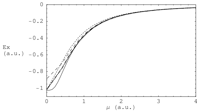
FIG. 9: Accurate short-range exchange energy of He (solid curve) along the erf-gau adiabatic connection, local density approximation (long-dashed curve) and three interpolations between the PBE value at \mu = 0 and the LDA at \mu \rightarrow \infty using a rational approximant (Eq. 38, short-dashed curve), a weighted approximant (Eq. 40, dotted curve) and the approximation of Iikura et al. (Eq. 43, dashed-dotted curve). The last two curves are nearly superimposed.
