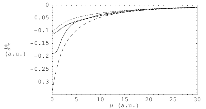
FIG. 14: Accurate short-range correlation energy of \text{Ne}^{6+} (solid curve) along the erf adiabatic connection, local density approximation (long-dashed curve) and two interpolations between the PBE value at \mu = 0 and the LDA at \mu \rightarrow \infty using a rational approximant (Eq. 39, short-dashed curve) and a weighted approximant (Eq. 41, dotted curve).
