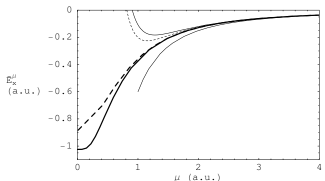
FIG. 5: Accurate short-range exchange energy of He (thick solid curve) along the erf-gau adiabatic connection, local density approximation (thick long-dashed curve), exact asymptotic expansion for \mu \rightarrow \infty (Eq. 28) with the first term (lower solid curve) and with the first two terms (upper solid curve), and asymptotic expansion in LDA (Eq. 33) with the first two terms (short-dashed curve), the first term in LDA being exact.
