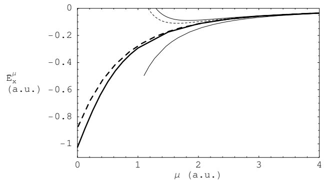
FIG. 4: Accurate short-range exchange energy of He (thick solid curve) along the erf adiabatic connection, local density approximation (thick long-dashed curve), exact asymptotic expansion for \mu \rightarrow \infty (Eq. 28) with the first term (lower solid curve) and with the first two terms (upper solid curve), and asymptotic expansion in LDA (Eq. 33) with the first two terms (short-dashed curve), the first term in LDA being exact.
