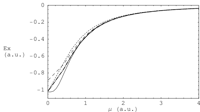
FIG. 9: Accurate short-range exchange energy of He (solid curve) along the erf-gau adiabatic connection, local density approximation (long-dashed curve) and three interpolations between the PBE value at \mu = 0 and the LDA at \mu \rightarrow \infty using a rational approximant (Eq. 38, short-dashed curve), a weighted approximant (Eq. 40, dotted curve) and the approximation of Iikura et al. (Eq. 43, dashed-dotted curve). The last two curves are nearly superimposed.
