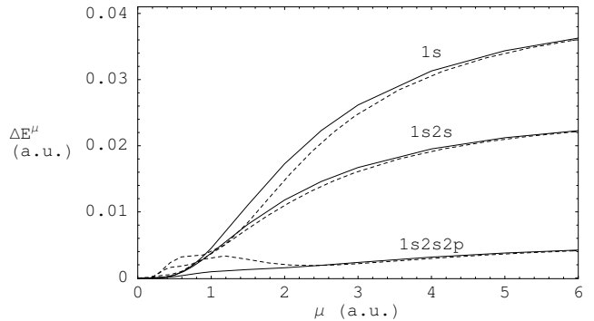
FIG. 2: Ground-state energy differences \Delta E_S^\mu = \langle \Psi_S^\mu | \hat{H}^\mu | \Psi_S^\mu \rangle - \langle \Psi^\mu | \hat{H}^\mu | \Psi^\mu \rangle where \Psi^\mu is an accurate wave function and \Psi_S^\mu are approximate wave functions generated from small orbital spaces S = 1s , S = 1s2s and S = 1s2s2p along the erf (full curves) and erf-gau (dashed curves) adiabatic connections for He.
