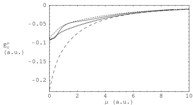
FIG. 13: Accurate short-range correlation energy of Be (solid curve) along the erfgau adiabatic connection, local density approximation (long-dashed curve) and two interpolations between the PBE value at \mu = 0 and the LDA at \mu \rightarrow \infty using a rational approximant (Eq. 39, short-dashed curve) and a weighted approximant (Eq. 41, dotted curve).
