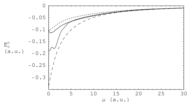
FIG. 15: Accurate short-range correlation energy of \text{Ne}^{6+} (solid curve) along the erfgau adiabatic connection, local density approximation (long-dashed curve) and two interpolations between the PBE value at \mu = 0 and the LDA at \mu \rightarrow \infty using a rational approximant (Eq. 39, short-dashed curve) and a weighted approximant (Eq. 41, dotted curve).
