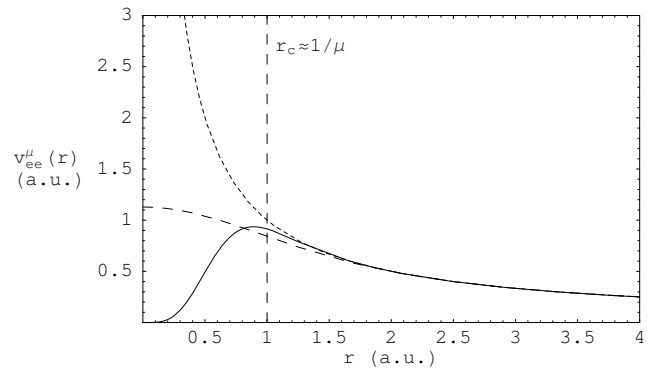
FIG. 1: Coulomb interaction 1/r (dotted curve), erf interaction (dashed curve) and erfgau interaction (solid curve) for \mu = 1 . In order to compare the two modified interactions, a scale factor is applied on the interaction parameter of the erfgau interaction: \mu \rightarrow c\mu with c = 3.375 (see text). It is possible to define a common cut-off radius r_c \approx 1/\mu .
