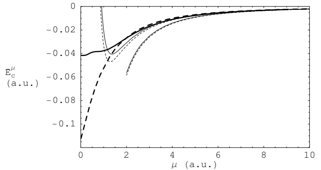
FIG. 7: Accurate short-range correlation energy of He (thick solid curve) along the erf-gau adiabatic connection, local density approximation (thick long-dashed curve), exact asymptotic expansion for \mu \rightarrow \infty (Eq. 30) with the first term (lower solid curve) and with the first two terms (upper solid curve), and asymptotic expansion in LDA (Eq. 34) with the first term (lower short-dashed curve) and with the first two terms (upper short-dashed curve).
