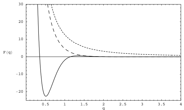
FIG. 6: Fourier transforms of the Coulomb interaction (dotted line), erf interaction (dashed line) and erfgau interaction (solid line), each plotted with an interaction parameter \mu = 0.5 .
