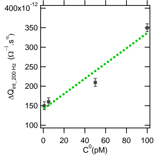
Figure 5 Calibration curve of the normalised \Delta Q_{\text{int,BSA,eq}} versus BSA concentration for ultralow concentration from 1 pM to 100 pM at fixed frequency 200 Hz.
