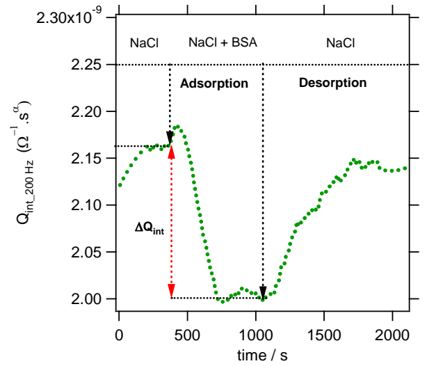
Figure 4. Sensorgrams showing Q_{\text{int}} change calculated using equation (12) with time for BSA adsorption and desorption steps at 200 Hz and a flow rate equal to 7.2 \mu\text{L}/\text{min} . Step 1: the 10^{-2} \text{ M} NaCl buffer was introduced for 360 s. Step 2: the diluted 1 pM BSA was introduced for 600 s for incubation. Step 3: the NaCl buffer was introduced again for the washing procedure for 1100 s.
