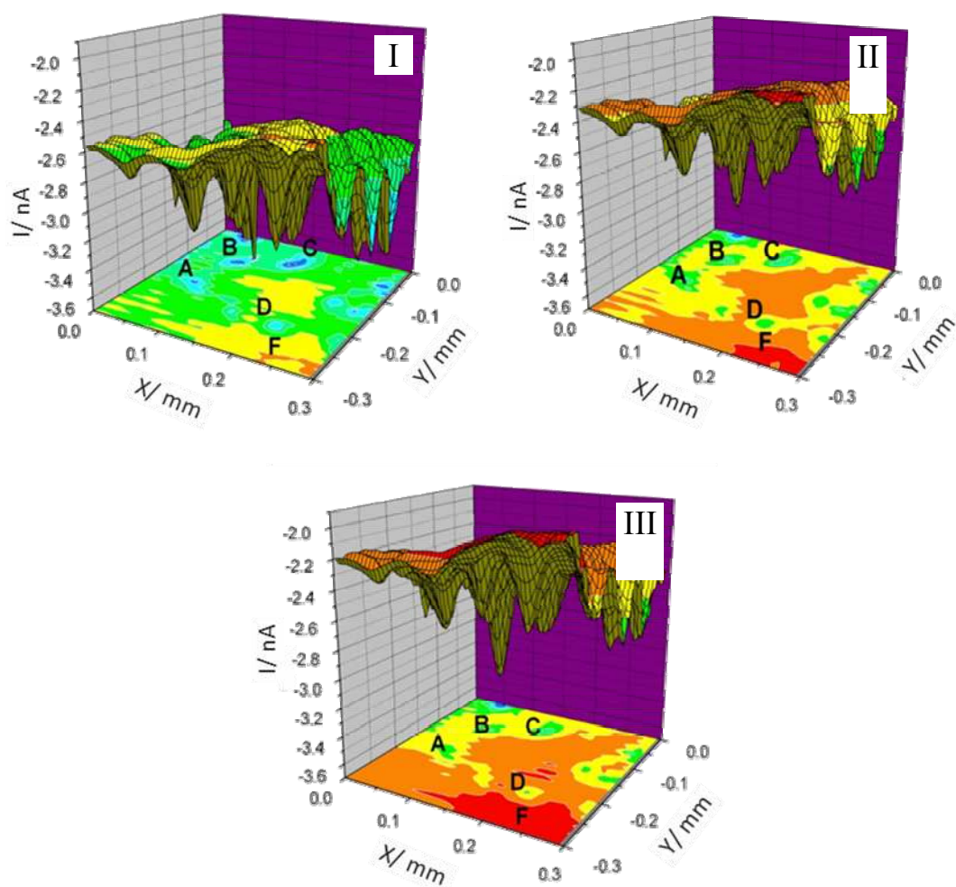
Figure 9. Topographic maps of the cement paste membrane obtained as a function of time. The downstream compartment solution containing 5 mM K_3Fe(CN)_6 + 0.01 M KCl. The downstream compartment solution containing 10 mM K_3Fe(CN)_6 + 0.5 M KCl. The diameter of the tip was \phi = 10 \mu m , the sweep rate v = 10 \mu m \cdot s^{-1} , L = 0.8 , and E_{tip} = -0.3V vs.SCE.
