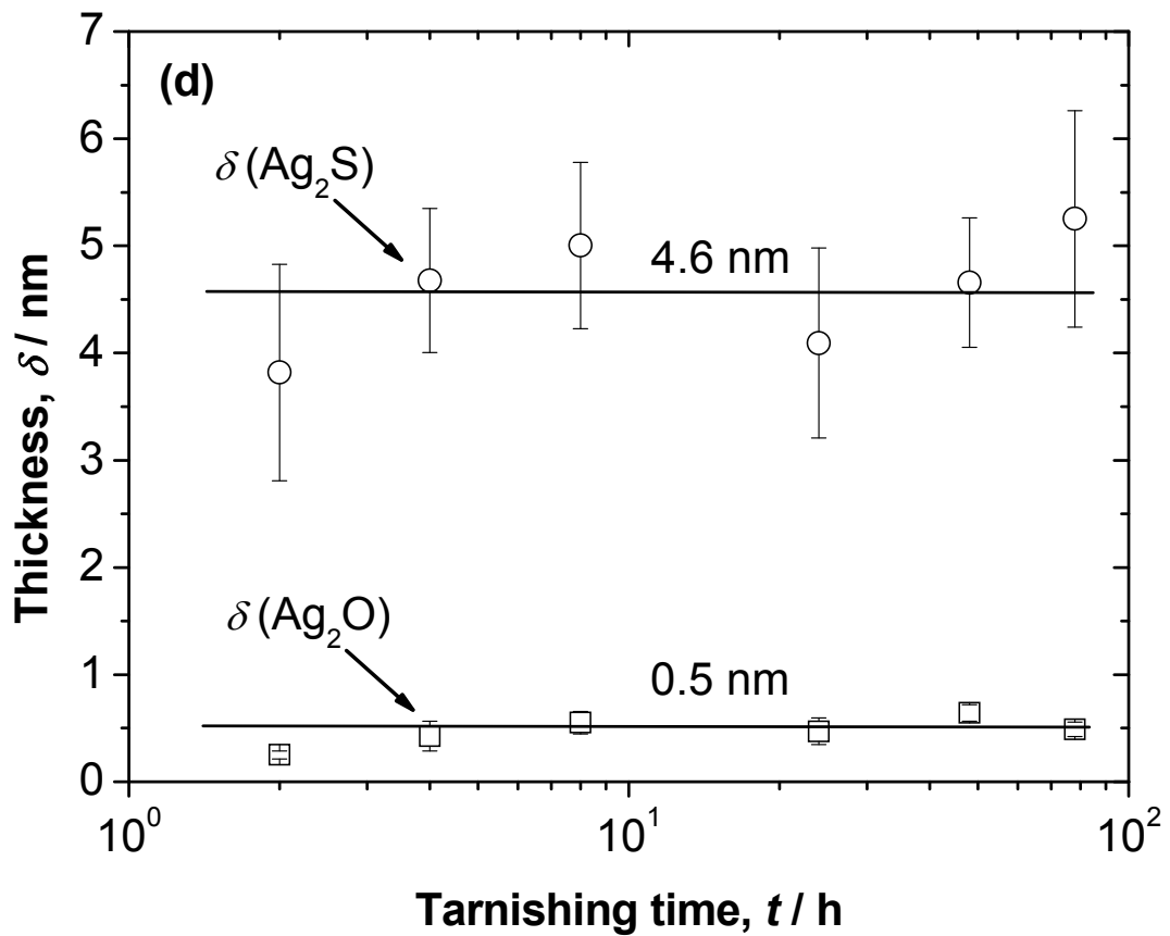
Fig. 7: Variation of the fitting parameters calculated from equations (10), (11), and (15).
