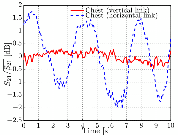
Figure 3: Channel fading amplitude for two measurement samples of S_{21} normalized by their mean values.
