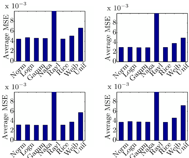
Figure 2: Average MSE of common distribution fits. The above row presents the vertical polarization and the below row presents the horizontal polarization. The left column is the vertical links while the right column is the horizontal links.
