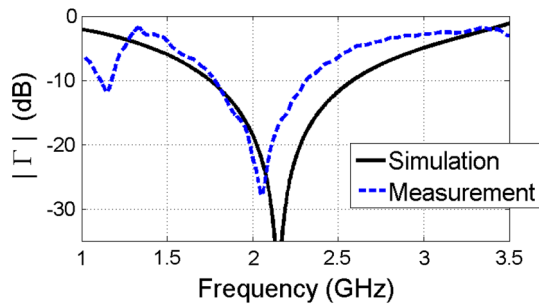
Fig. 10 Comparison between simulation and measurement results at oblique incidence ( 65^\circ ). TM polarization
