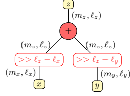
Fig. 5. Fixed-point adder
