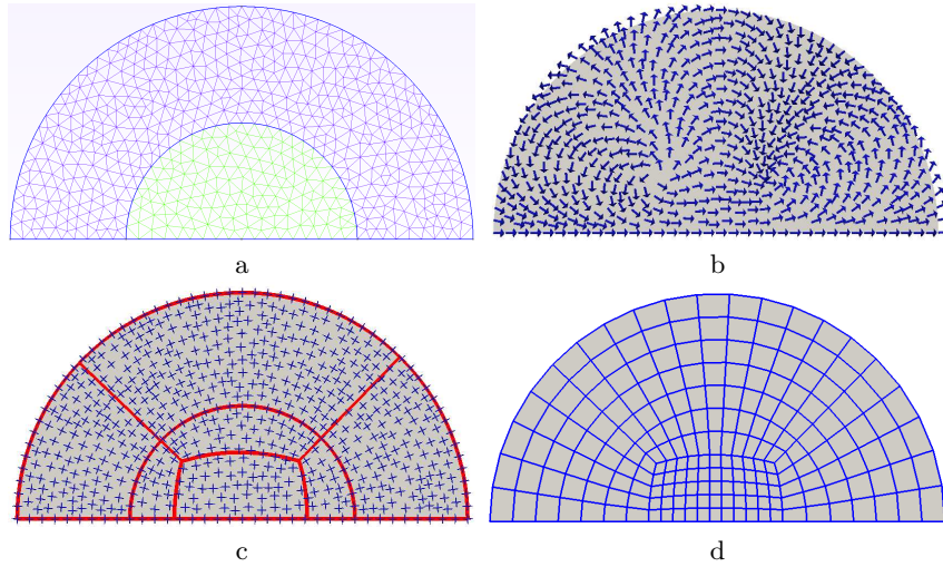
Fig. 1. Overview of the main steps of our algorithm. In a , the background mesh used. The geometry has two domains with distinct mesh colors. In b , the unit representation vector field obtained by solving a PDE. In c , the corresponding cross field and the domain partitioning into four-sided regions. In d , a full quadrilateral mesh is obtained by using a bilinear transfinite interpolation over each region.
