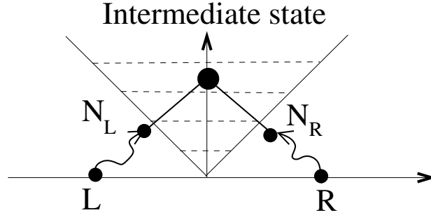
Figure 2: Schematic of the modified Riemann solver (30). The New-left and New-right states are modification of the initial Left and Right states.
