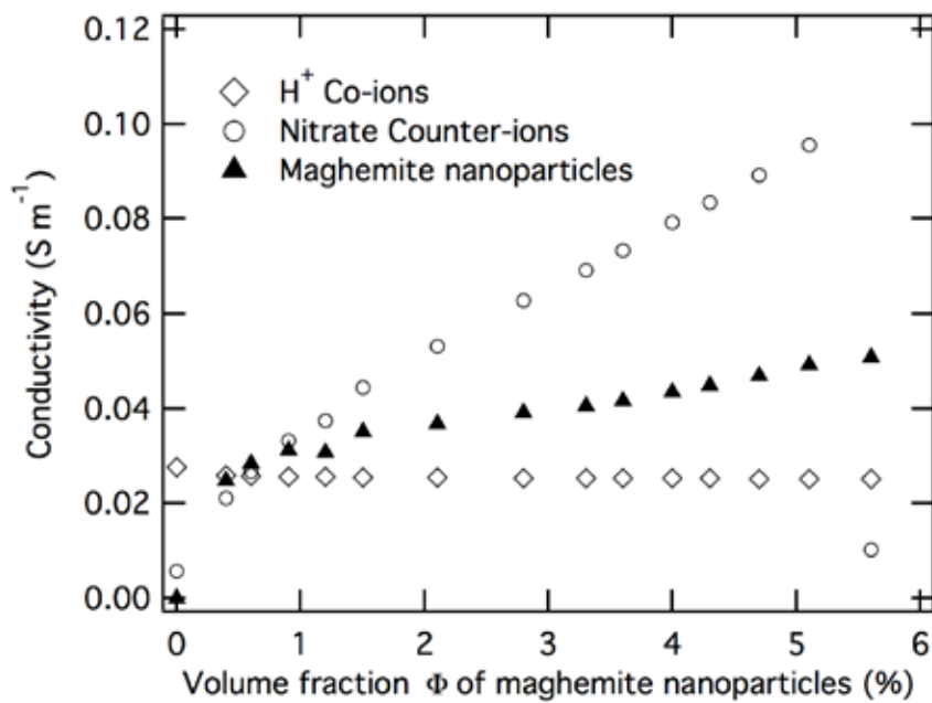
Figure 3: Contribution to the electrical conductivity of the different charged species as a function of the volume fraction \mathbf{f} of maghemite nanoparticles as computed by the MSA-transport theory. Nanoparticles surrounded by adsorbed counterions, bearing a dynamic effective charge (full triangles), free \text{NO}_3^- counterions (empty circles) and \text{H}^+ co-ions (empty diamonds).
