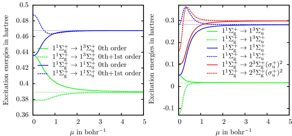
Figure 4: Zeroth-order \Delta \mathcal{E}_k^\mu (plain line) and zeroth+first-order \Delta E_k^{\mu,(0+1)} (dashed line) excitation energies of the hydrogen molecule (in hartree) as a function of \mu in bohr -1 at the equilibrium distance (left) and three times the equilibrium distance (right). The excitation energies of the physical system \Delta E_k are plotted as horizontal dotted lines.
