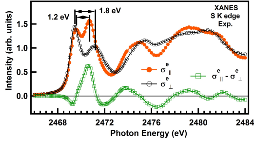
Figure 3: Polarization dependence in the near S K edge region. The difference of the intensities, \sigma_{\parallel}^e - \sigma_{\perp}^e , the linear dichroism, is shown by green squares.
