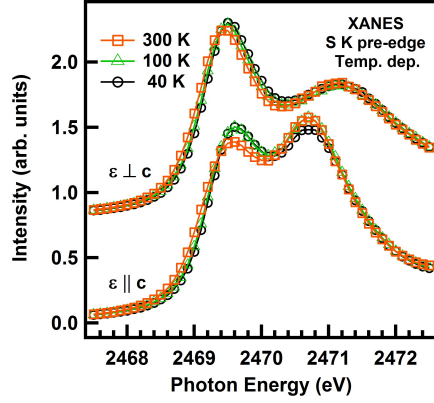
Figure 5: Temperature dependence of the two pre-edge features for the two orientations, \epsilon \parallel c and \epsilon \perp c , shifted vertically for clarity.
