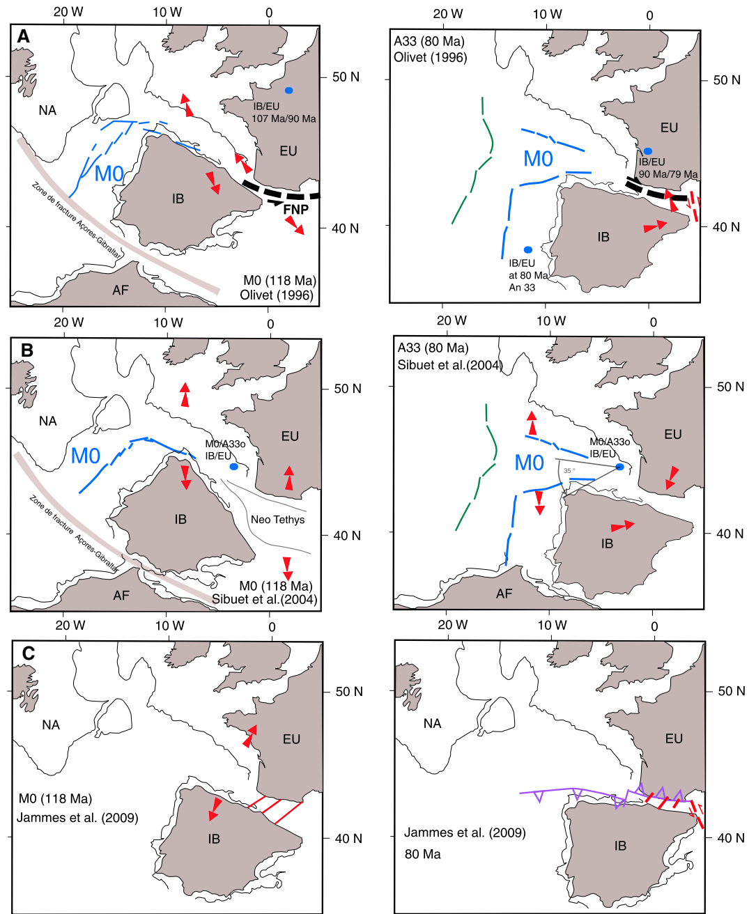
Figure 2. Proposed kinematic reconstructions of Iberia motion in the Lower Cretaceous ( M_0 anomaly \sim 118 Ma) and at onset of convergence in Late Cretaceous (anomaly An33 at 80 Ma). (a) Transtensional rift model after Olivet [1996], which accounts for dextral strike-slip reactivation and inversion of the Iberian and European margins during oblique convergence. (b) Kinematic reconstruction of Mesozoic motion of Iberia after Jammes et al. [2009] that includes transcurrent motion of Iberia during the Late Jurassic, followed by orthogonal stretching in the Middle-Late Cretaceous, and subsequent frontal convergence of Iberia. (c) Scissor opening model after Srivastava et al. [2000] that implies large oceanic subduction beneath the Pyrenees during the Albian. The position of North America (NA), Africa (AF), and Iberia (IB) relative to fixed Eurasia (EU) is shown as well as location of IB/EU rotation poles (blue circles). Anomaly A33 and M_0 are shown as green and blue segments, respectively.
