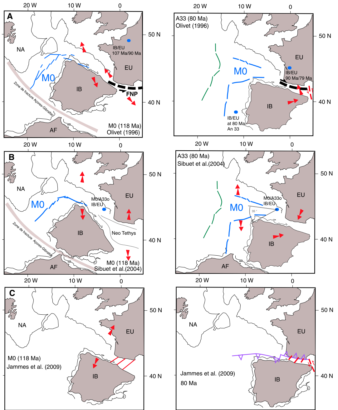
Figure 2. Proposed kinematic reconstructions of Iberia motion in the Lower Cretaceous ( M_0 anomaly \sim 118 Ma) and at onset of convergence in Late Cretaceous (anomaly A33 at 80 Ma). (a) Transtensional rift model after Olivet [1996], which accounts for dextral strike-slip reactivation and inversion of the Iberian and European margins during oblique convergence. (b) Kinematic reconstruction of Mesozoic motion of Iberia after Jammes et al. [2009] that includes transcurrent motion of Iberia during the Late Jurassic, followed by orthogonal stretching in the Middle-Late Cretaceous, and subsequent frontal convergence of Iberia. (c) Scissor opening model after Srivastava et al. [2000] that implies large oceanic subduction beneath the Pyrenees during the Albian. The position of North America (NA), Africa (AF), and Iberia (IB) relative to fixed Eurasia (EU) is shown as well as location of IB/EU rotation poles (blue circles). Anomaly A33 and M_0 are shown as green and blue segments, respectively.
