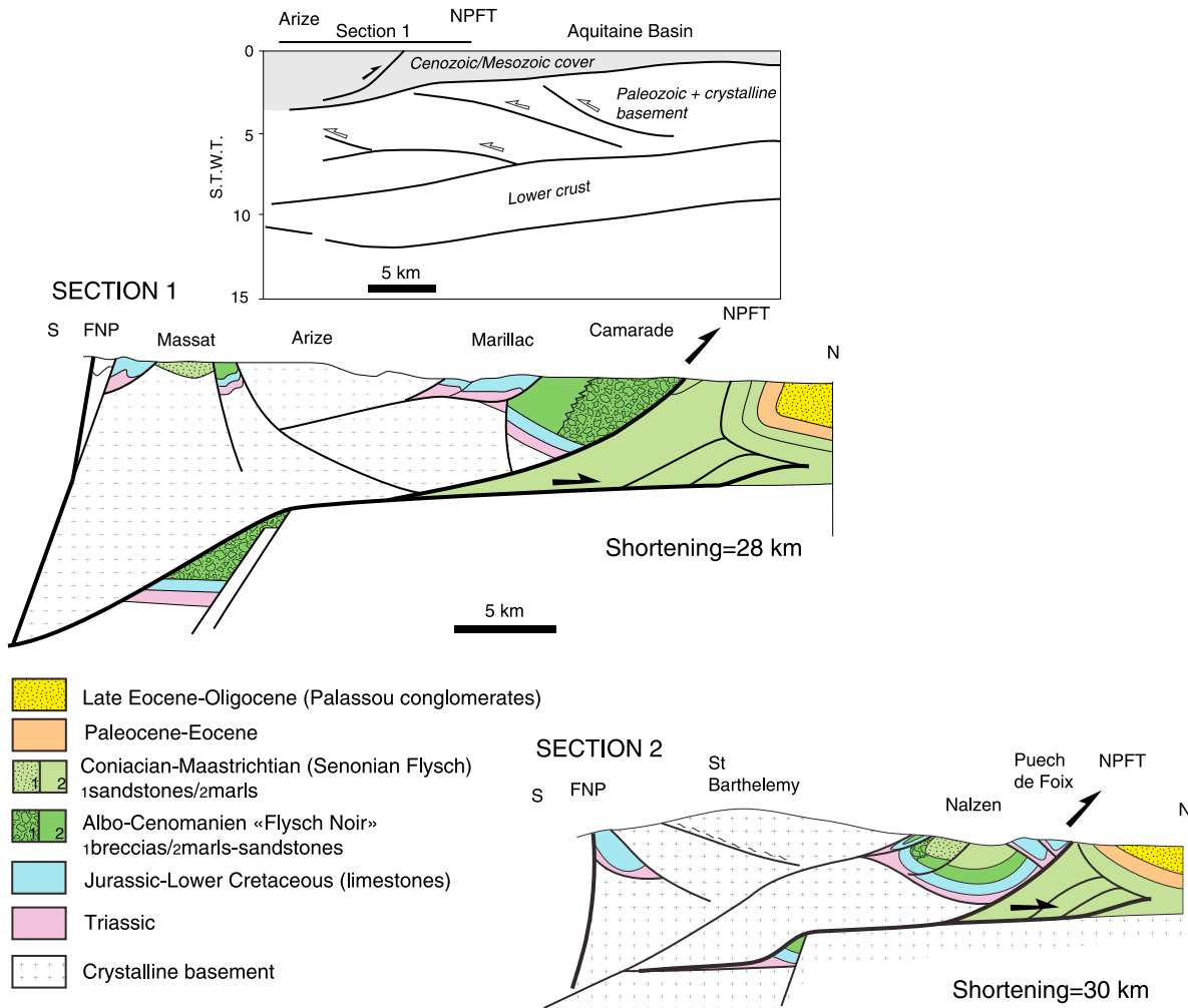
Figure 6. Geological balanced sections across the northern Pyrenees redrawn after Baby [1988] (location in Figure 5) and line drawing from interpretation of the ECORS profile parallel to section 1 [ Choukroune et al. , 1990] showing the north facing Variscan thrusts negatively inverted during the Permian. The sections outline an overall thick-skinned style with prominent basement-involved shortening. According to the interpretation of the ECORS profile [ Baby , 1988; Roure et al. , 1989; Muñoz , 1992], the NPFT is a low-angle, south dipping, crustal thrust ramp rooting into the layered lower crust or the mantle.
