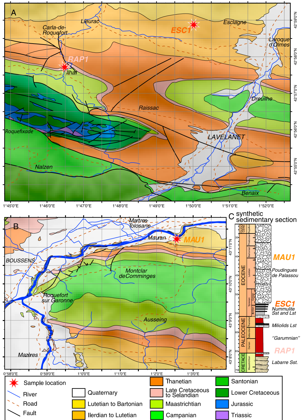
Figure 7. Sampling sites for U/Pb, ZHe, and AFT analyses in the northern Pyrenees (location of maps in Figure 1). Samples RAP1, ESC1, and MAU1 are replaced on a generic lithostratigraphic section.
