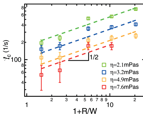
Fig. 3 Critical shear rate ( \dot{\gamma}_c ) as a function of the normalized radius ( 1 + R/W ) for solutions of PEO 2Mio at a concentration of 400 ppm for different solvent viscosities ( \eta_s ). The dotted lines represent fits to the data using eqn (3). Each experiment was repeated at least two times using fresh polymer solutions and the average value is shown together with the error bars.
