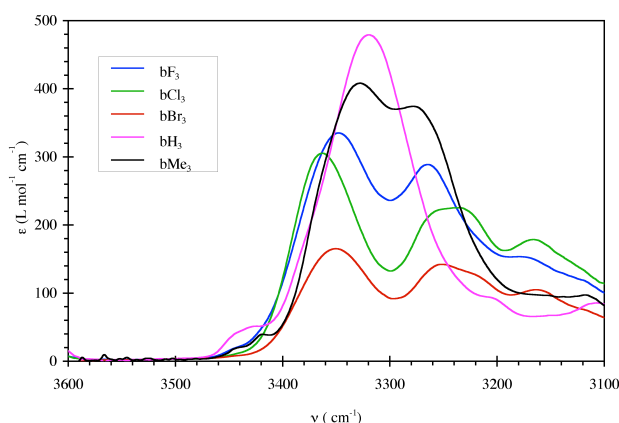
Fig. 1 FTIR spectra for bis-ureas at 10^{-2} \text{ mol/L} in chloroform ( 20^\circ\text{C} ).
