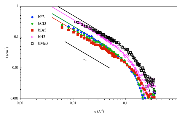
Fig. 2 SANS intensity ( I ) versus scattering vector ( q ) for bis-urea solutions in \text{CDCl}_3 at 15 \text{ g/L} (ca 0.03 \text{ mol/L} ) and 22^\circ\text{C} . The plain curves are fits according to a model for long rigid filaments with a circular cross-section (characteristic dimensions in Table S3).
