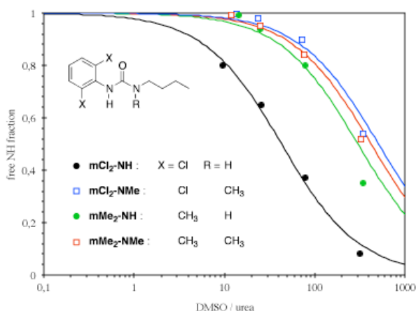
Fig. 4 Free N-H fraction determined by FTIR for mixtures of mono-ureas ( 5 \cdot 10^{-3} mol/L) and DMSO in chloroform (20°C). The curves are fits to a 1:1 association model.
