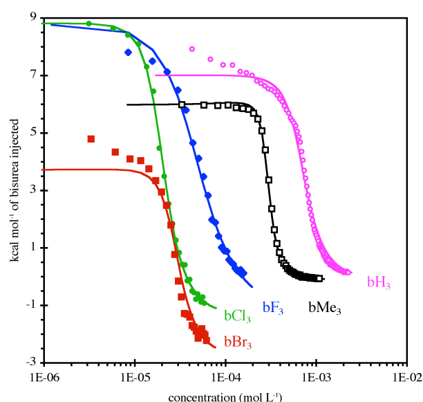
Fig. 3 ITC enthalpograms for bis-urea solutions in chloroform injected into chloroform versus total bis-urea concentration in the cell ( T = 20^\circ\text{C} ).
