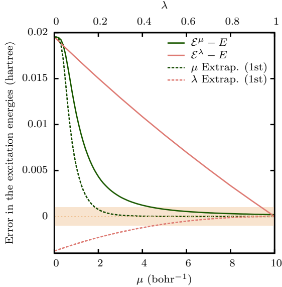
Figure 5: Error in the ^3\text{S} excitation energy along the range-separated and linear adiabatic connections for the helium atom as functions of \mu and \lambda . The unextrapolated energies are given in full lines and the extrapolated ones in dashed lines. An error smaller than 1 mhartree around the physical limit is given by the colored region.
