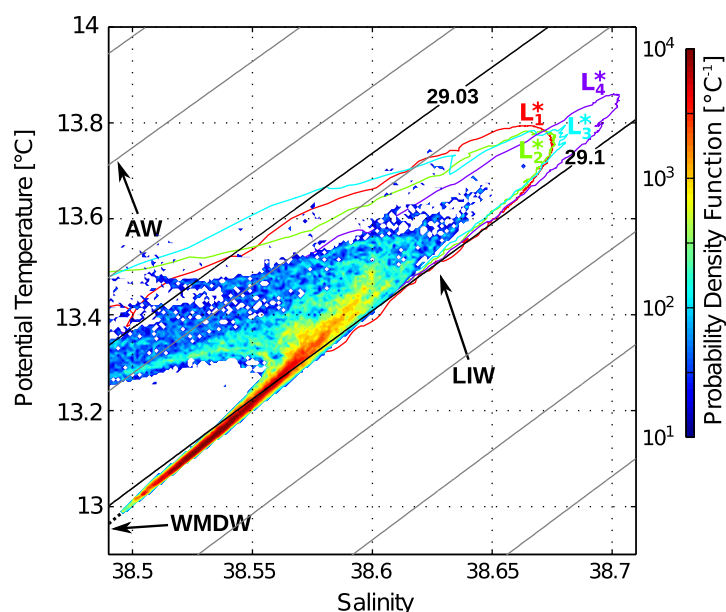
Figure 4. Volumetric \theta/S diagram with the main water masses (AW, LIW, and WMDW) made up by all the profiles (down to 1000 m) collected during the four glider deployments revealing the SCV L_1^* . The empirical probability density function was normalized such as its integral in the \theta/S space equals to unity. The colored lines labeled by L_i^* are associated with the profiles carried out within the core of the four SCVs. Slanted lines represent isopycnals.
