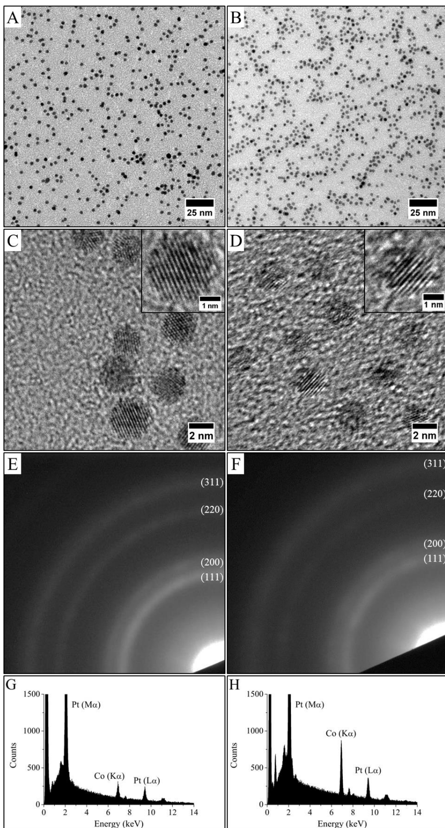
Figure 2: TEM images (A-B), HRTEM images (C-D), electronic diffraction (E-F) and EDX analysis (G-H) of (Co_{30}Pt_{70})_{Polyol} (left images) and (Co_{50}Pt_{50})_{Polyol} (right images).
