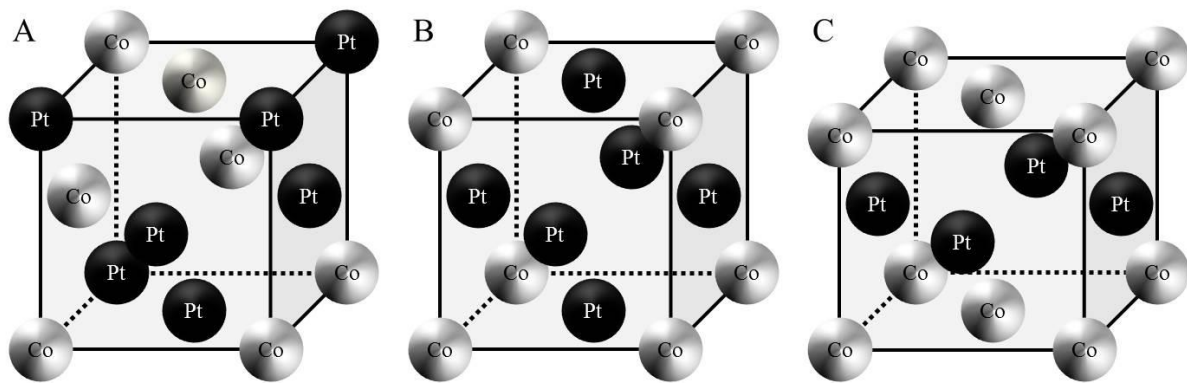
Figure 1 : Representation of Co_xPt_{100-x} structure in three different phases: (A) disordered phase A1 with cubic symmetry (B) ordered phase L1_2 with cubic symmetry ( X=25 ) and (C) ordered phase L1_0 with face centered tetragonal symmetry ( X=50 ).
