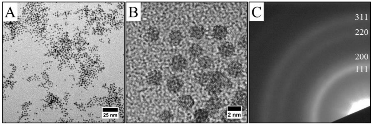
Figure 3: TEM images (A), HRTEM images (B) and electronic diffraction (C) of (\text{Co}_{30}\text{Pt}_{70})_{\text{LLPT}}
