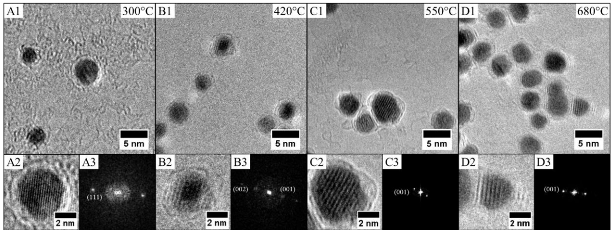
Figure 5: HRTEM images of (\text{Co}_{30}\text{Pt}_{70})_{\text{Polyol}} at various annealing temperatures: (A) 300°C; (B) 420°C; (C): 550°C and (D) 680°C. For each temperature, HRTEM images of one nanoparticle (A2, B2, C2, D2) and the associated FFT (A3, B3, C3, D3).
