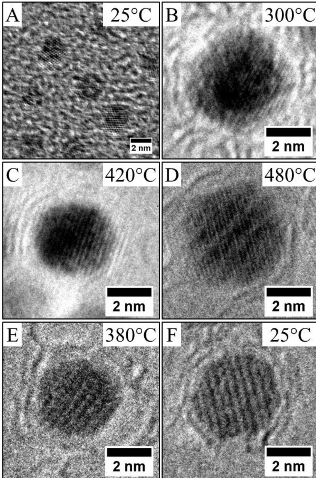
Figure 8: HRTEM images of (\text{Co}_{50}\text{Pt}_{50})_{\text{polyol}} during annealing treatment: (A) room temperature (RT), (B) 300°C, (C) 420°C on the increasing part of the annealing and (D) 480°C, (E) 380°C and (F) RT on the decreasing part of the annealing.
