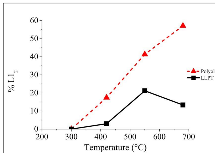
Figure 6: Evolution of ordering with temperature during the annealing process.
