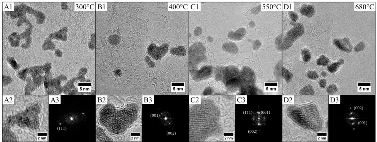
Figure 7: HRTEM images of (\text{Co}_{30}\text{Pt}_{70})_{\text{LLPT}} at various annealing temperatures: (A) 300°C; (B) 400°C; (C): 550°C and (D) 680°C. For each temperature, HRTEM images of one nanoparticle (A2, B2, C2, D2) and the associated FFT (A3, B3, C3, D3).
