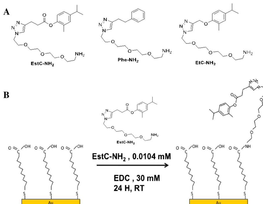
Figure 1 Structures of the carvacrol derivatives grafted on gold surfaces (A). Schematic representation of the two consecutive steps leading to the immobilization of EstC-NH 2 on Au surface, via esterification of the acidic functions of MUA by EDC (B).
