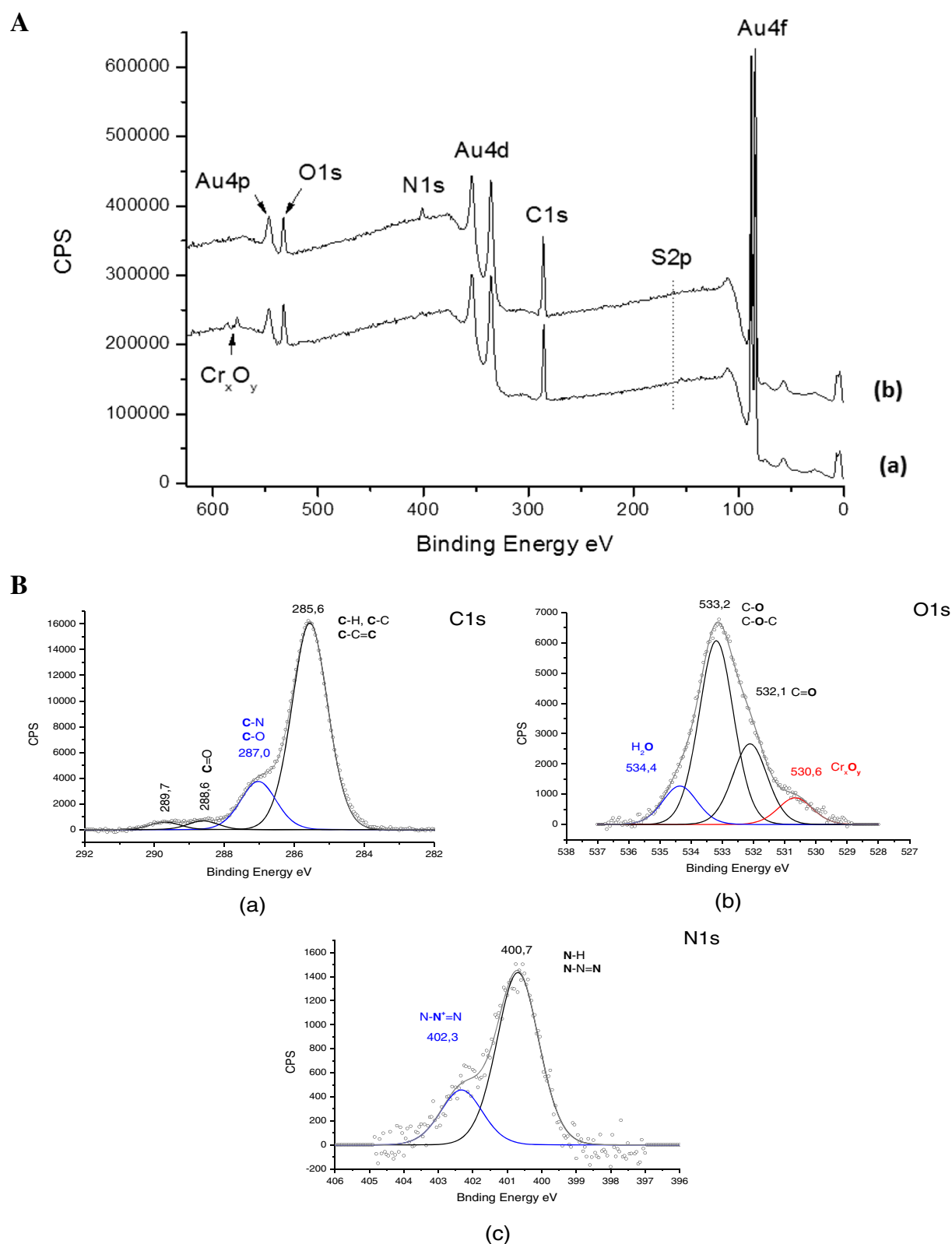
Figure 3 XPS general spectra of gold surfaces. A: XPS general spectra of gold surfaces functionalized (a) only with MUA (control) or (b) with the EstC-NH 2 molecule. B: XPS high-resolution spectra of gold EstC-NH 2 functionalized-surfaces for Carbon (a), for Oxygen (b) and for Nitrogen (c).
