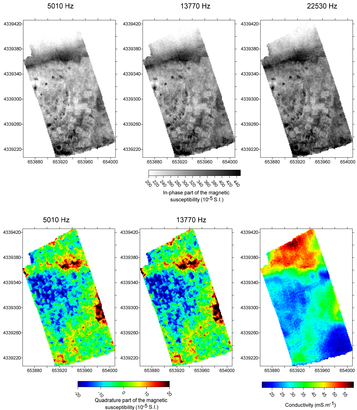
Figure 2 Map of the GEM-2 processed data: On the top, maps of the in-phase components of the magnetic susceptibility, for 5010 Hz, 13770 Hz and 22530 Hz. On the bottom, maps of the quadrature components of the magnetic susceptibility for 5010 and 13770 Hz and of the conductivity (to the right). We observe an increase of the in phase susceptibility offset at the different frequencies. The quadrature components of the magnetic susceptibility, in accordance with the theory, are non-dependent of the frequency.
