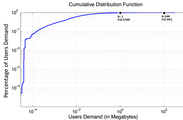
Figure 4: Cumulative Distribution Function of users demands.
