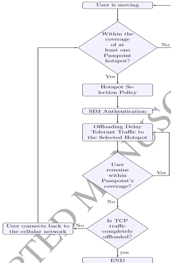
Figure 5: Offloading algorithm.
