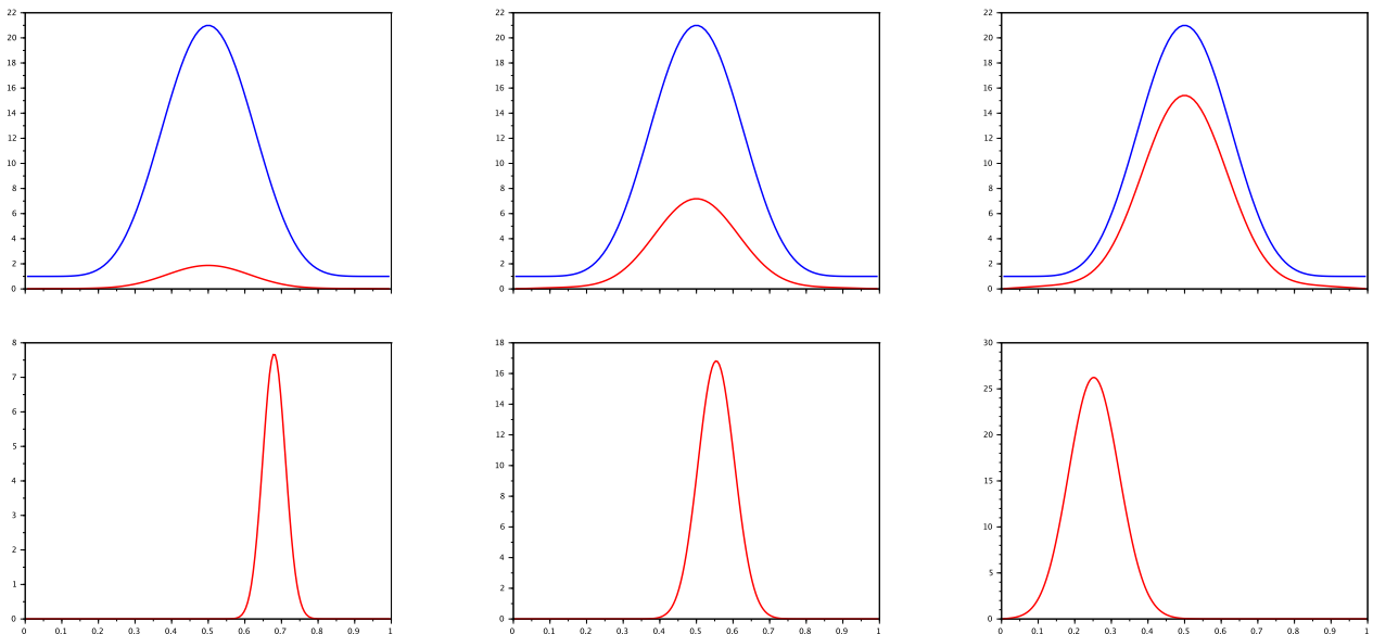
Figure 1: Snapshots of the evolution of the dispersal for three different times according to the parabolic problem (28). Top figures depict the space repartition \rho(x) (fixed blue curve = K , increasing red = \rho ). Bottom figures depict the trait distribution \int_0^1 n(x, \theta, t) dx .
