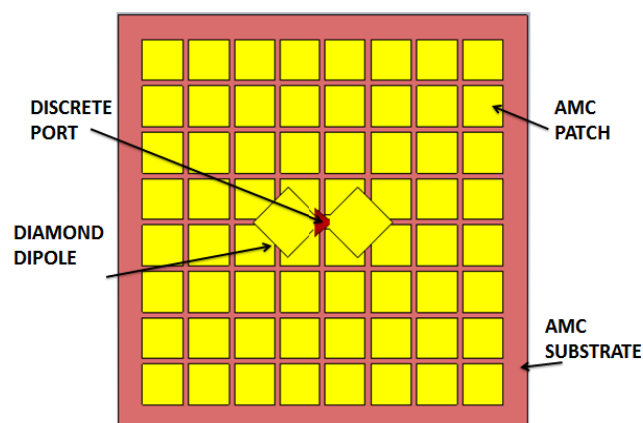
Fig. 2. Antenna with Classical AMC Reflector.
