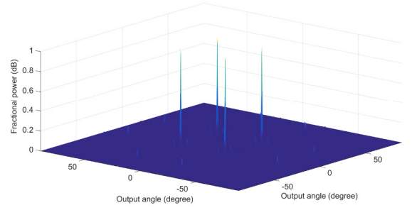
Figure 5 : Far field beam pattern with 4 pixels
