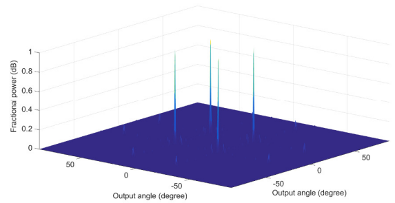
Figure 5 : Far field beam pattern with 4 pixels
